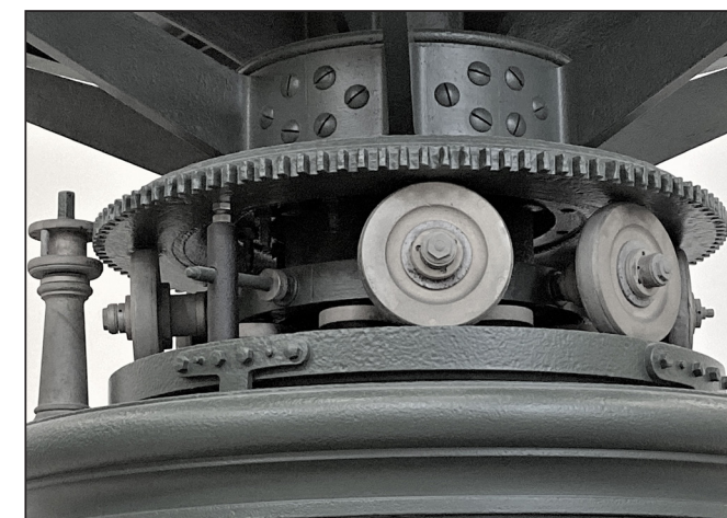
Clockwork mechanisms from the 1854 Fresnel lens.
